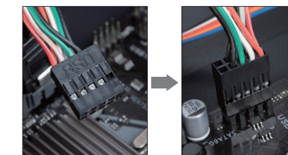
USB 2.0 connector / Conector USB 2.0
